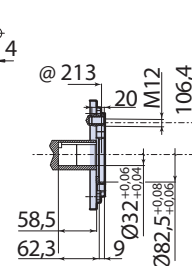
AR 500 bp Twin AR 560 bp Twin
